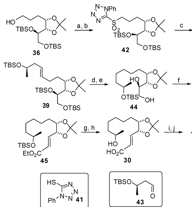
Scheme 6 Reagents and conditions: (a) 41 , DIAD, \text{PPh}_3 , THF, -20^\circ\text{C} , 92%; (b) (\text{NH}_4)_6\text{Mo}_7\text{O}_{24}\cdot 4\text{H}_2\text{O} , 30% \text{H}_2\text{O}_2 , EtOH, rt, 88%; (c) 43 , LiHMDS, THF, -78^\circ\text{C} , 83%; (d) \text{H}_2 , Pd/C, EtOH, rt, 2 h, 84%; (e) TBAF (1 M sol n in THF), THF, 0^\circ\text{C} , 2 h, 80%; (f) i) silica supp. \text{NaIO}_4 , \text{CH}_2\text{Cl}_2 , 0^\circ\text{C} , 1 h; ii) (\text{OEt})_2\text{P}(\text{O})\text{CH}_2\text{COOEt} , LiCl, DIPEA, THF, 6 h, 64% (for two steps); (g) LiOH, THF–MeOH– \text{H}_2\text{O} , 4 h, 93%; (h) TBAF (1 M sol n in THF), THF, 55^\circ\text{C} , 81%; (i) 2,4,6-trichlorobenzoyl chloride, \text{Et}_3\text{N} , THF, 2 h, then DMAP, toluene, reflux, 8 h, 71%; (j) TFA, \text{CH}_3\text{CN} – \text{H}_2\text{O} , 0^\circ\text{C} , 1 h, 65%.
