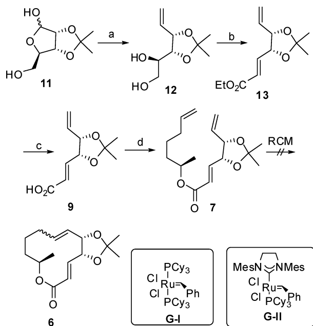
Scheme 1 Reagents and conditions: (a) Ph 3 PCH 2 Br, KO t Bu, THF, 0 °C, 80%; (b) i) silica supp. NaIO 4 , CH 2 Cl 2 ; ii) (OEt) 2 P(O)CH 2 CO 2 Et, NaH, THF, 0 °C, 87% (for two steps); (c) LiOH, THF/MeOH/H 2 O; (d) 8 , 2,4,6-trichlorobenzoyl chloride, Et 3 N, toluene, DMAP, 46% (for two steps).
